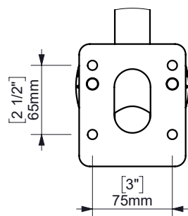
WALL FIXATION / ANCLAJE PARED
