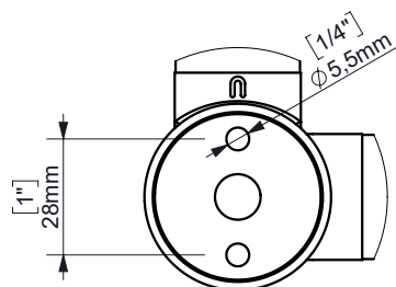
WALL FIXATION / ANCLAJE PARED
